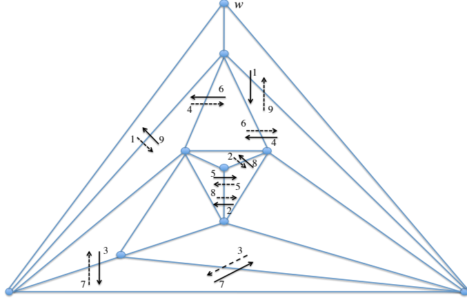
Fig. 2. Bold and dashed arrows indicate the pivots made by the exchange algorithm to get from R_0 to R'_0 and from R'_0 to R_0 , with the chosen special vertex w . As an example, bold arrow labelled by 1 has tail in room wef and head in room fie : it indicates that, in the first pivot (to get from R_0 to R'_0 ) room wfe is replaced by room fie .
