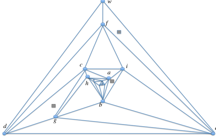
Fig. 3. The manifold (V_1, M_1) . Gray squares indicate the triangles corresponding to the initial room-partitioning R_1 .
