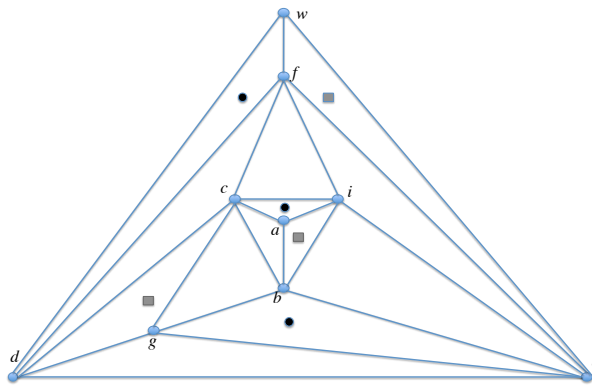
Fig. 1. The manifold (V_0, M_0) .
